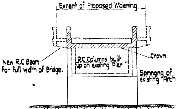
Fig. 209.—Widening by Double Cantilever on Columns built up from existing Piers.
